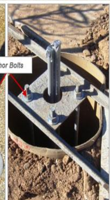
Concrete foundation pole
